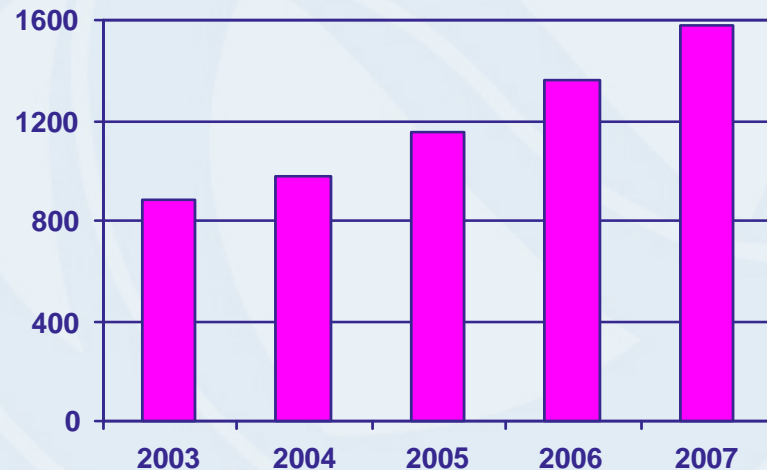
Members - Total
