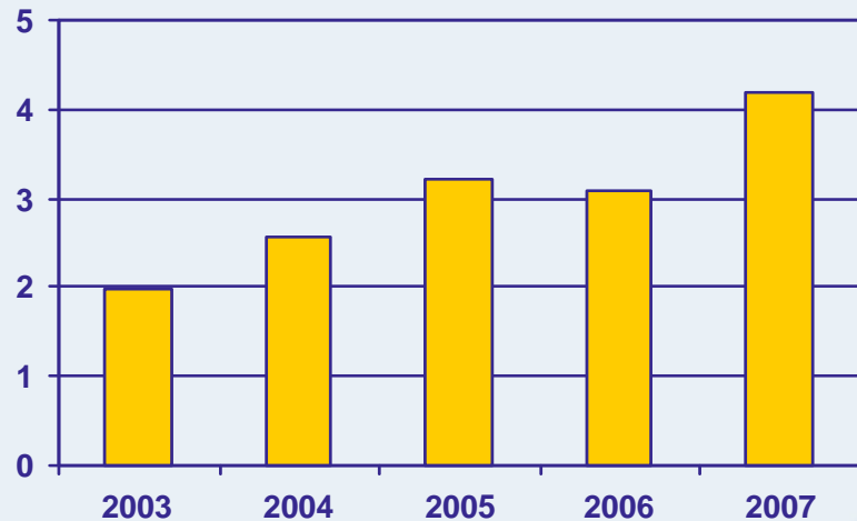
IPv4 - /8s
