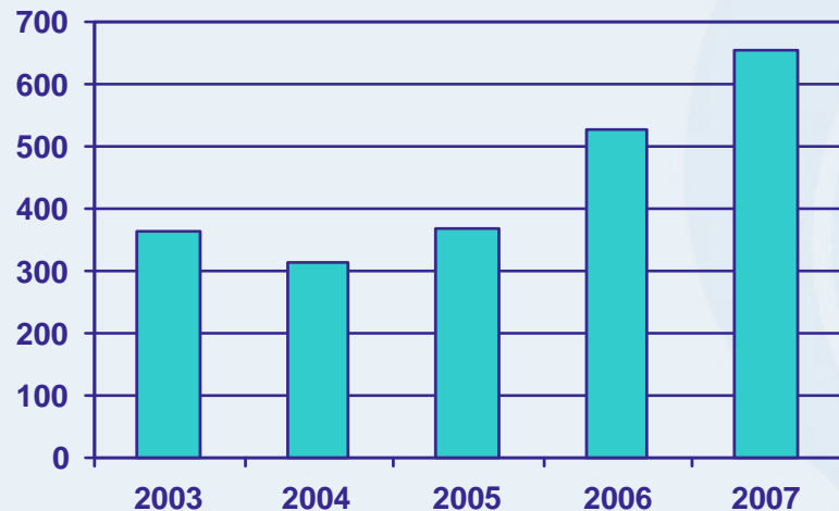
ASNs - Total
